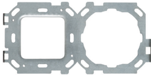
FOXXA01-71XX Metal mounting double frame for device + socket 71+55 or 71+45
