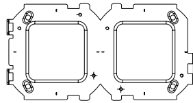
FOXXA01-6060 Metal mounting double frame for sockets 60+60
