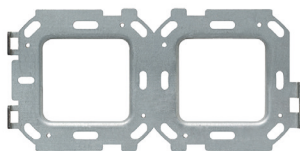
FOXXA01-7171 Metal mounting double frame for devices - 2X71
